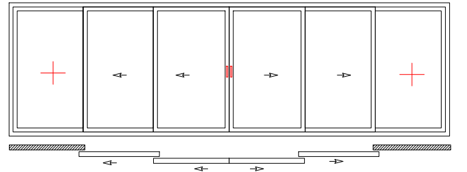
4 HAREKETLİ 2 SABİT KANAT 4 SLIDING 2 FIX SASH
